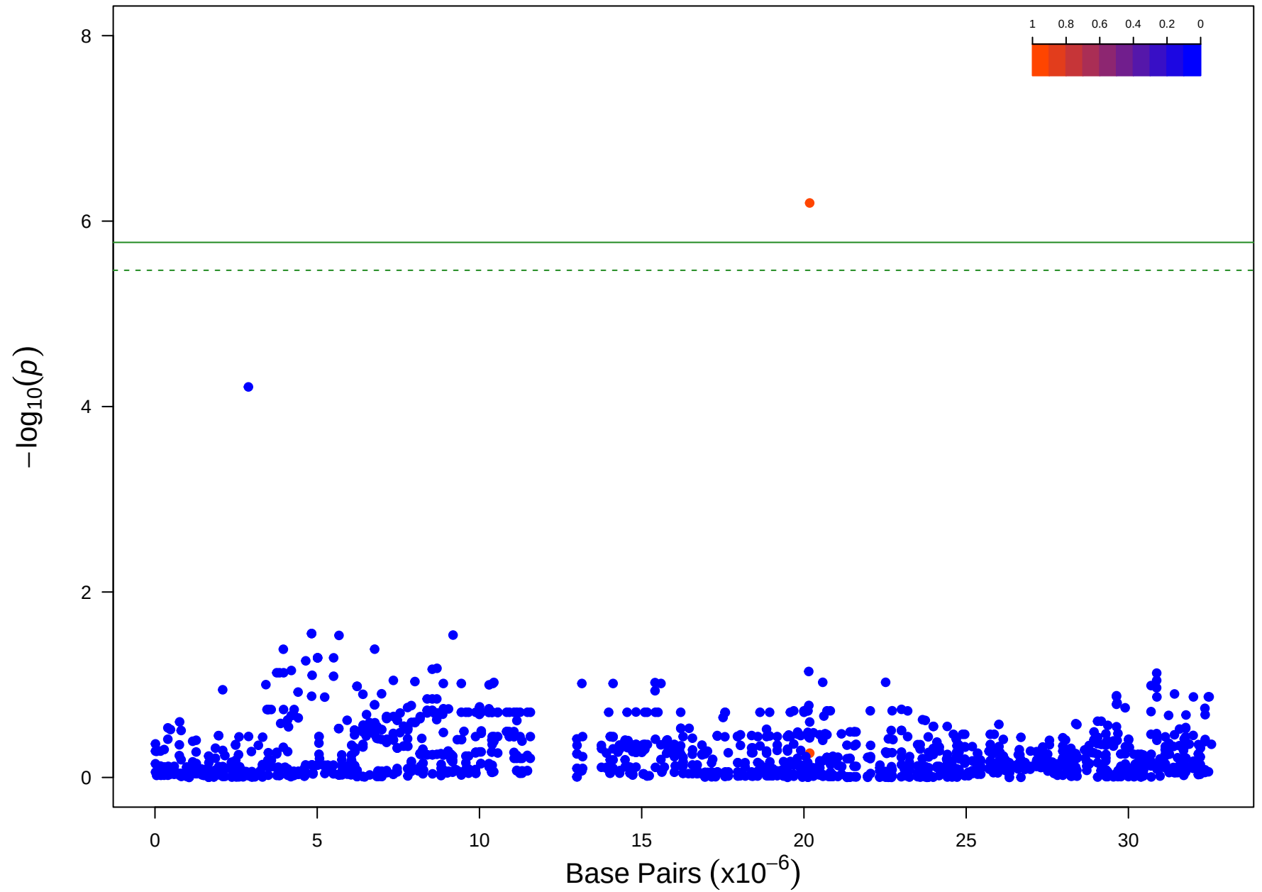
Chromosome 14
